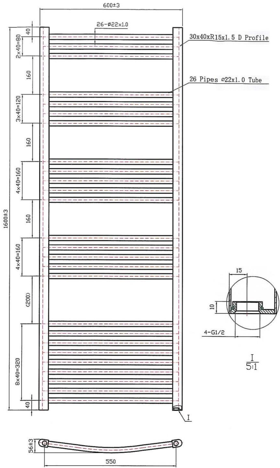
1600*600 26 pipes Curved
