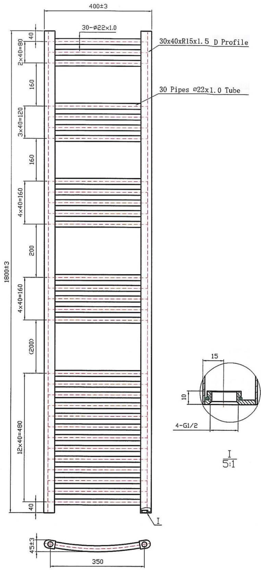
1800*400 30 pipes Curved
