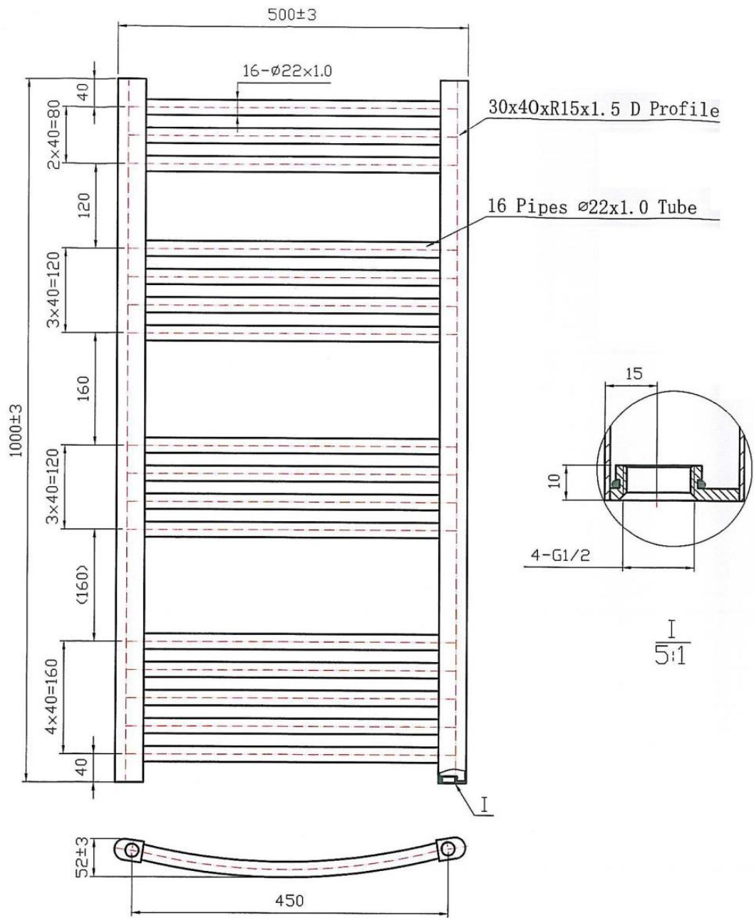
1000*500 16 pipes Curved
