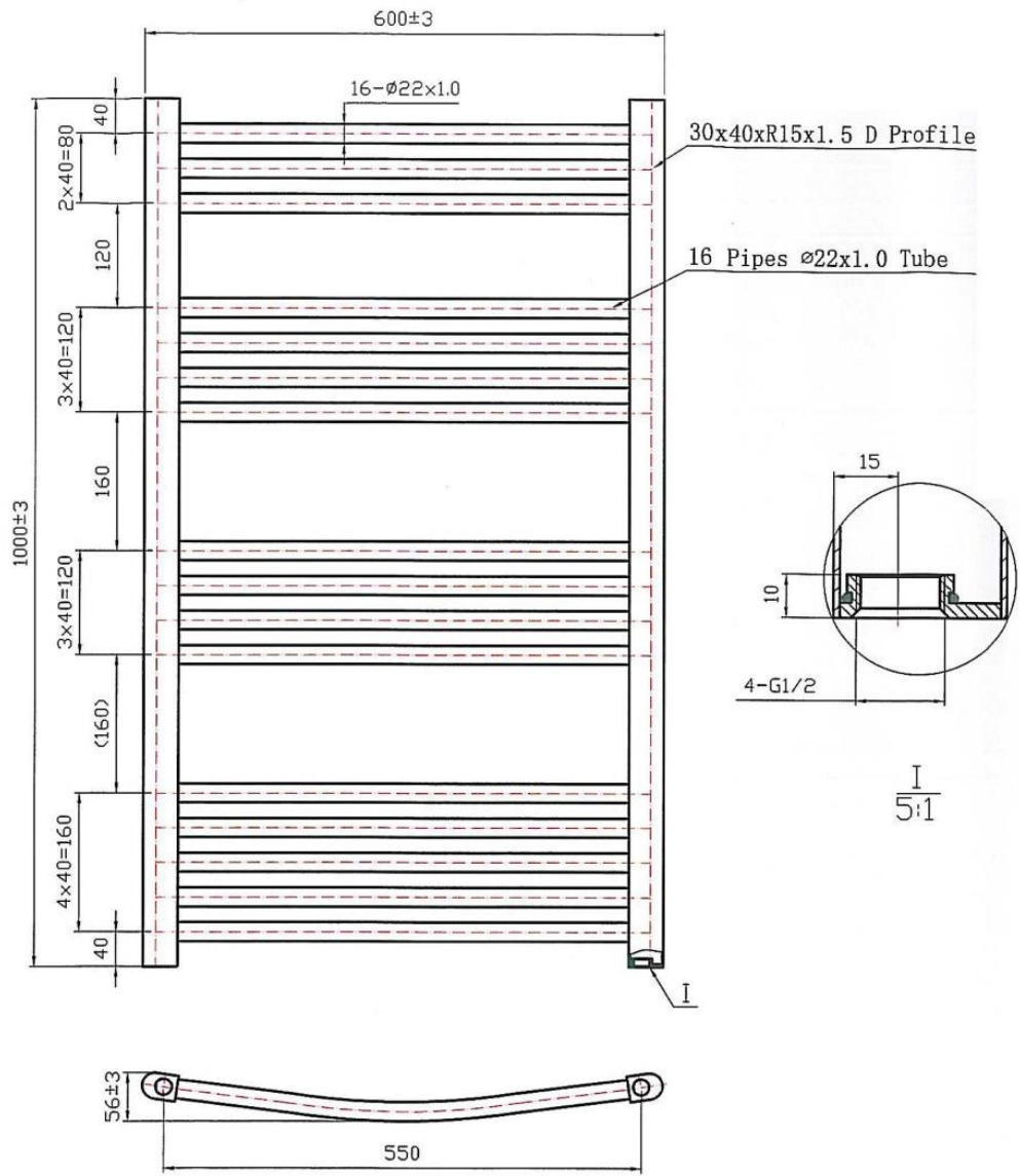
1000*600 16 pipes Curved
