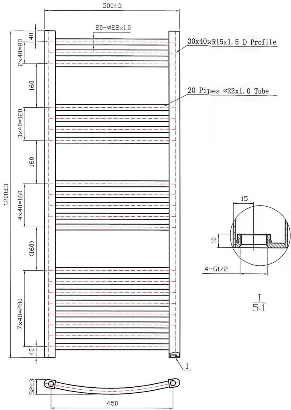
1200*500 20 pipes Curved
