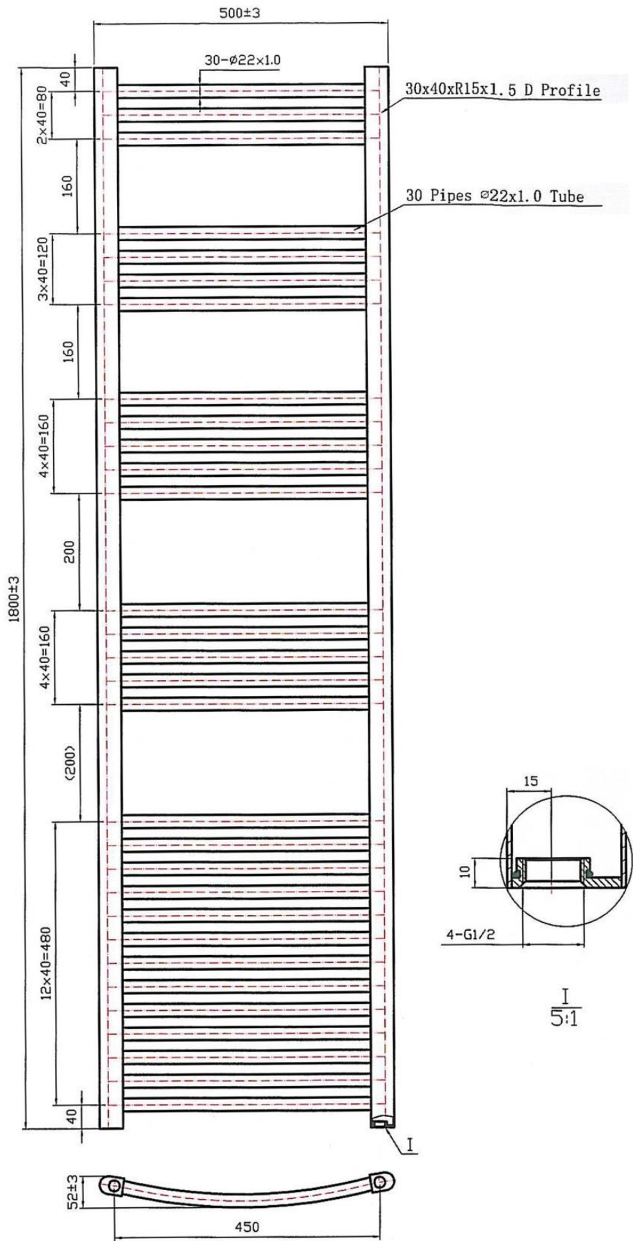
1800*500 30 pipes Curved
