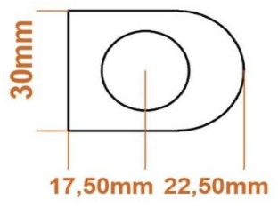
B SECTION
