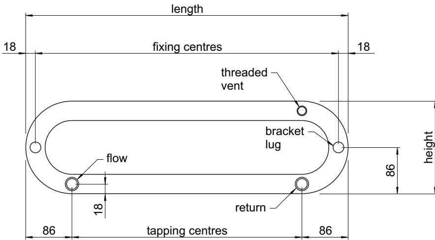
View on Rear of Radiator
